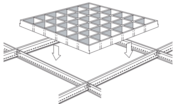
150mm x 150mm Cells
