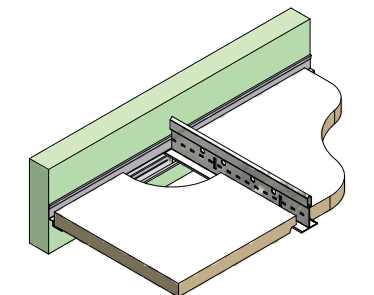
Wall Angle position is dropped to level of face of Panel; Tee Grid is packed at Wall Angle and Panel is square cut at wall angle
