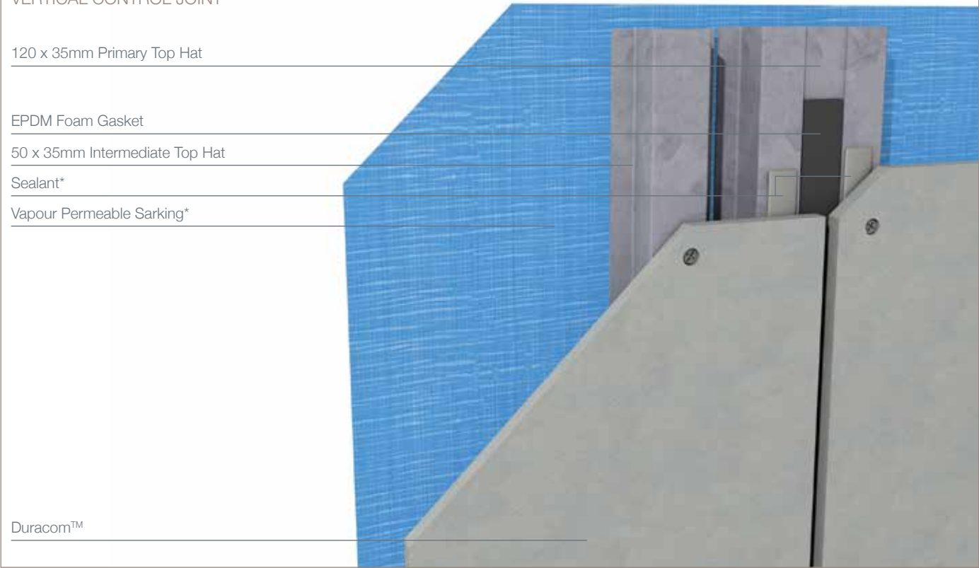
FIGURE 25 VERTICAL CONTROL JOINT
