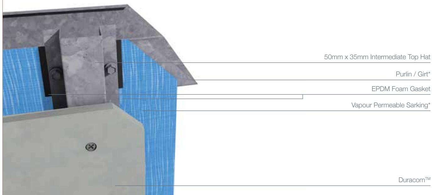
FIGURE 28 THERMAL BREAK
