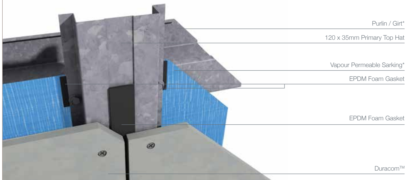
FIGURE 28 THERMAL BREAK
